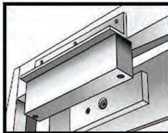
L-bracket for narrow door frame
