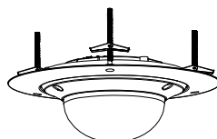
1241ZJ In-ceiling Mount
